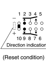
1-coil latching
