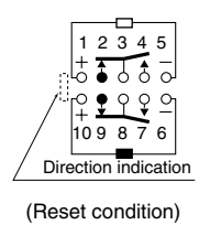
2-coil latching
